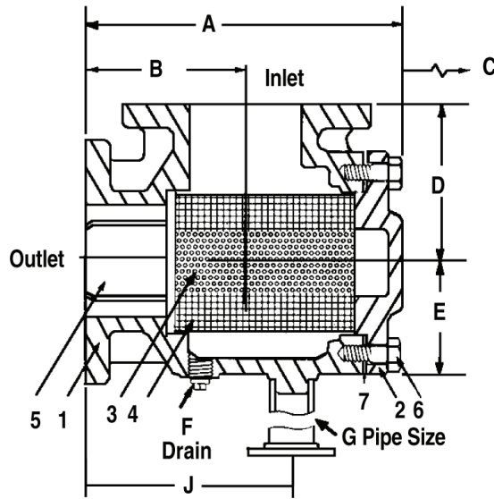
Dimensions - Inches (mm)
